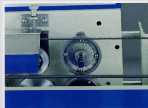
Employs two blades to trim package after sealing for neat edge.
